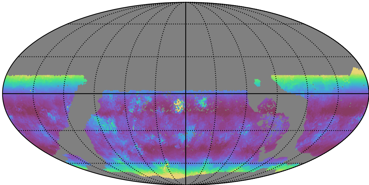
too_elab_r32_d3_griz_v3.4_10yrs WFD g band: Median airmass
