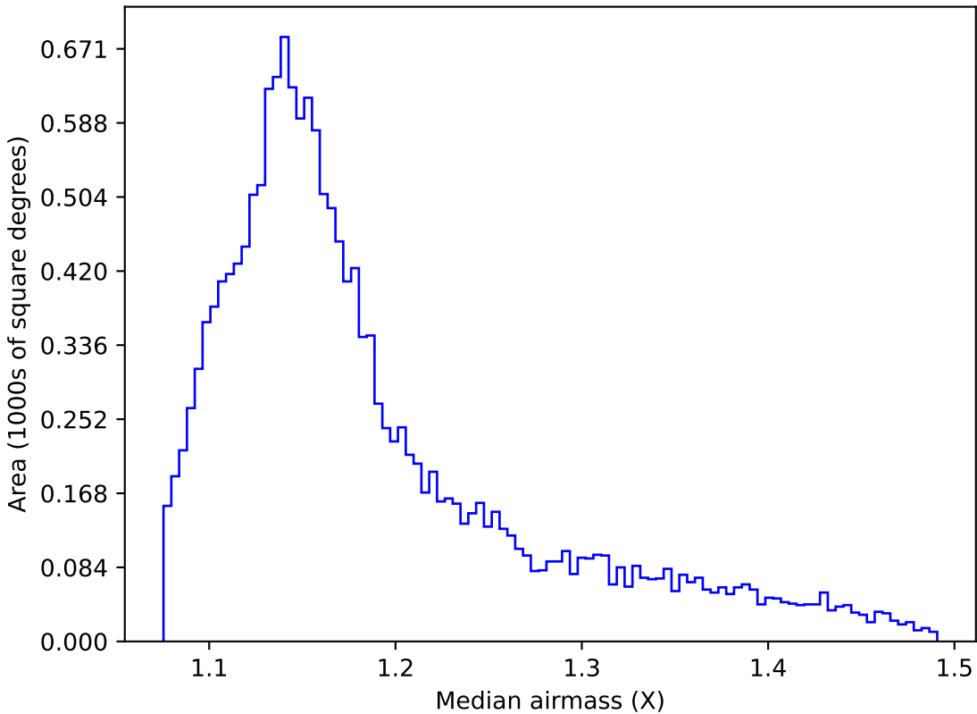
too_elab_r32_d3_griz_v3.4_10yrs WFD g band: Median airmass
