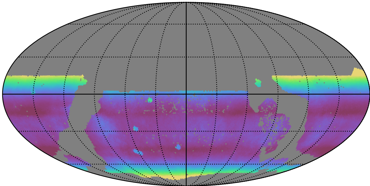
too_elab_r32_d3_griz_v3.4_10yrs WFD all bands: Median airmass
