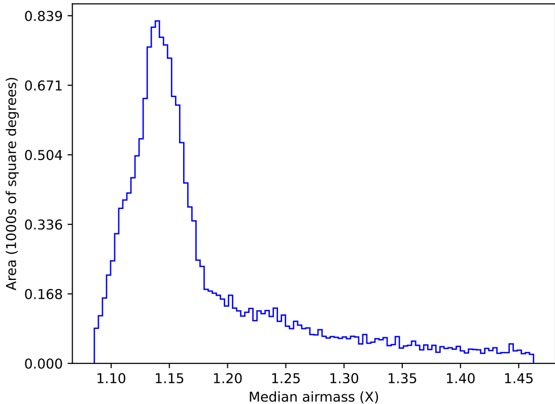
too_elab_r32_d3_griz_v3.4_10yrs WFD all bands: Median airmass
