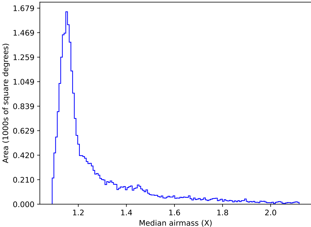
too_elab_r32_d3_griz_v3.4_10yrs All sky z band: Median airmass
