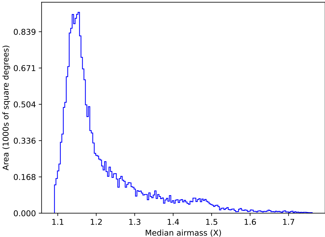
too_elab_r32_d3_griz_v3.4_10yrs All sky y band: Median airmass
