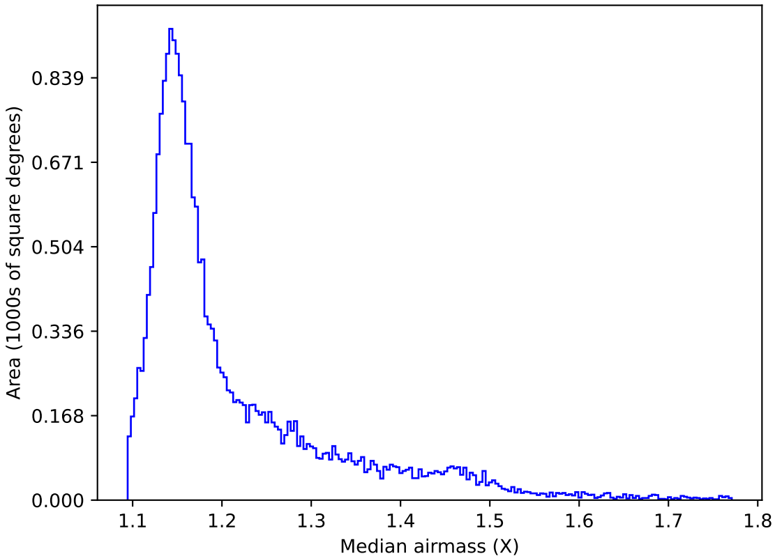
too_elab_r32_d3_griz_v3.4_10yrs All sky y band: Median airmass
