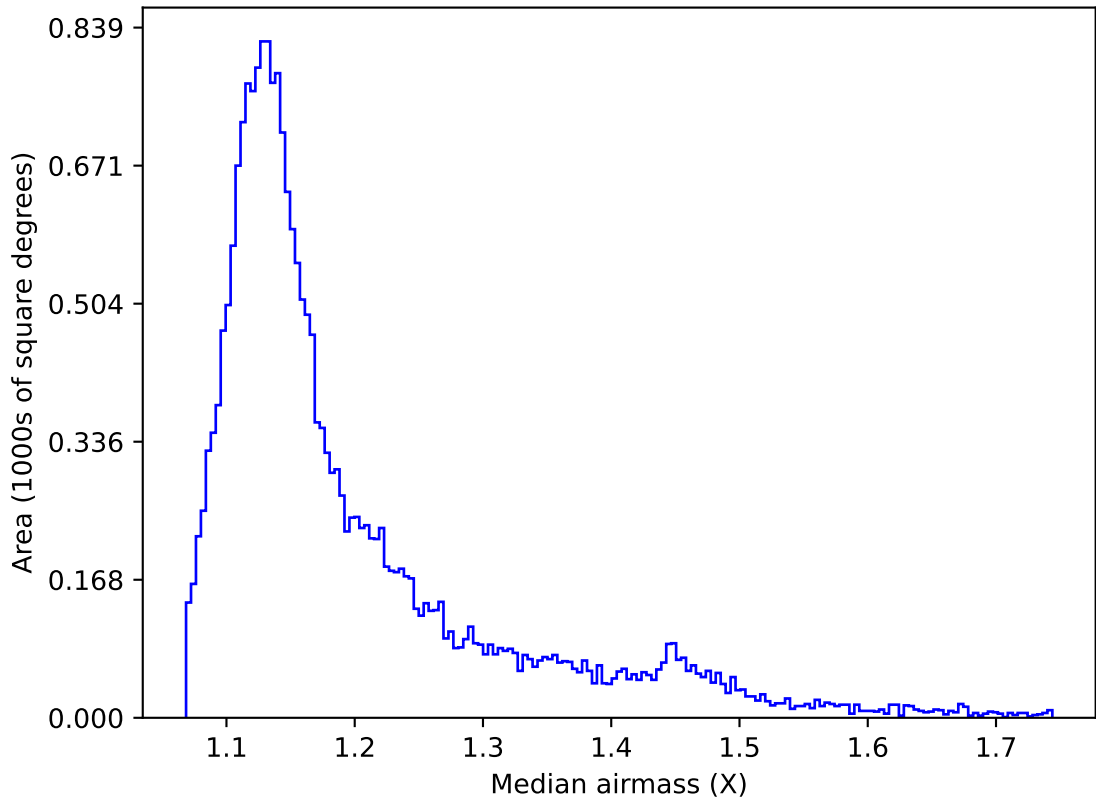
too_elab_r32_d3_griz_v3.4_10yrs All sky u band: Median airmass
