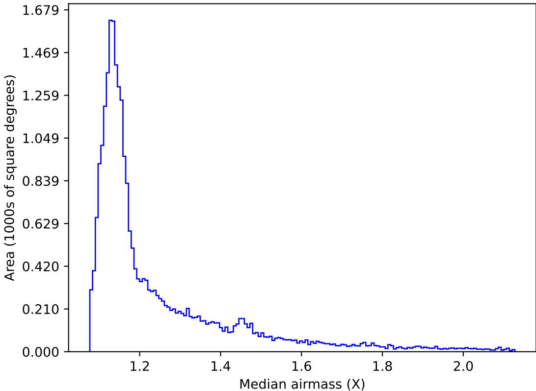
too_elab_r32_d3_griz_v3.4_10yrs All sky r band: Median airmass
