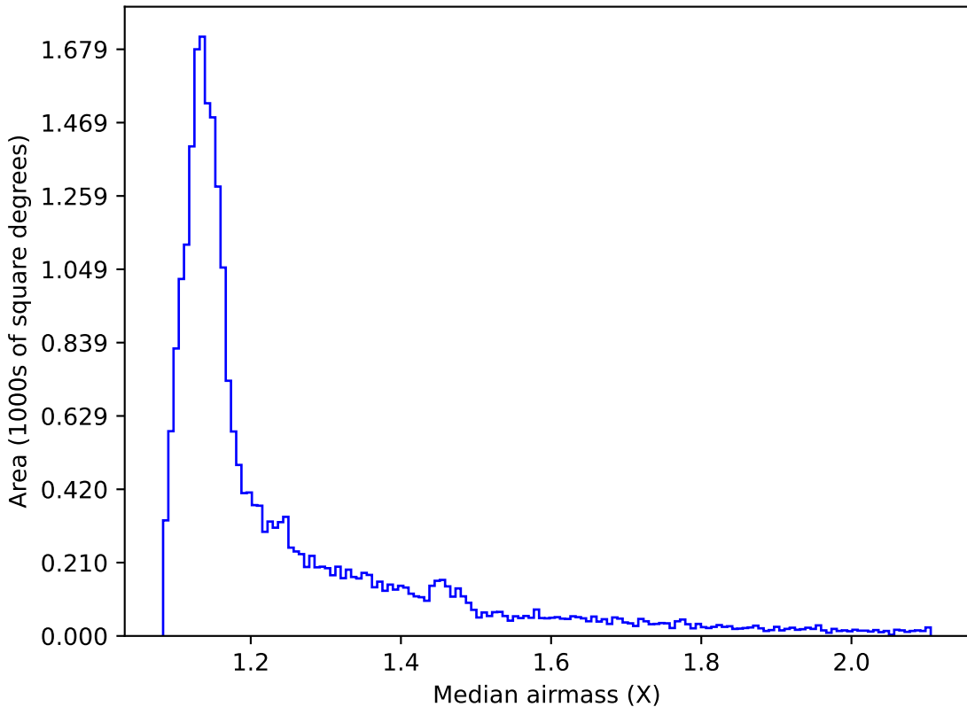
too_elab_r32_d3_griz_v3.4_10yrs All sky i band: Median airmass
