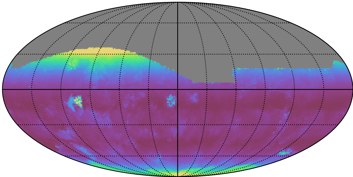
too_elab_r32_d3_griz_v3.4_10yrs All sky g band: Median airmass
