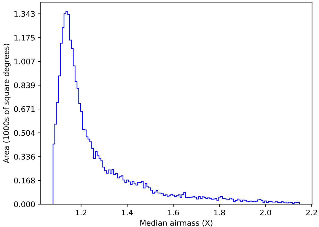
too_elab_r32_d3_griz_v3.4_10yrs All sky g band: Median airmass
