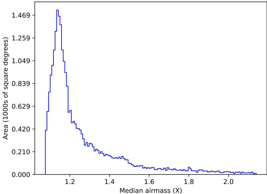
too_elab_r32_d3_griz_v3.4_10yrs All sky g band: Median airmass
