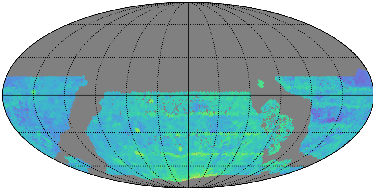
too_elab_r32_d3_griz_v3.4_10yrs WFD z band: Median Season Length
