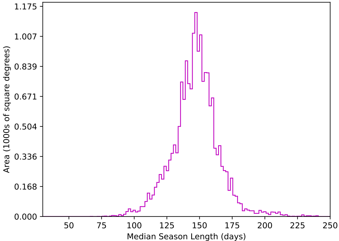
too_elab_r32_d3_griz_v3.4_10yrs WFD z band: Median Season Length
