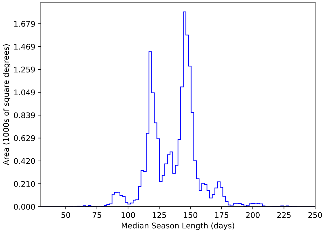
too_elab_r32_d3_griz_v3.4_10yrs WFD y band: Median Season Length
