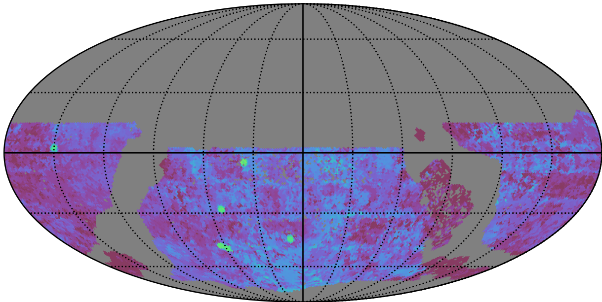
too_elab_r32_d3_griz_v3.4_10yrs WFD u band: Median Season Length
