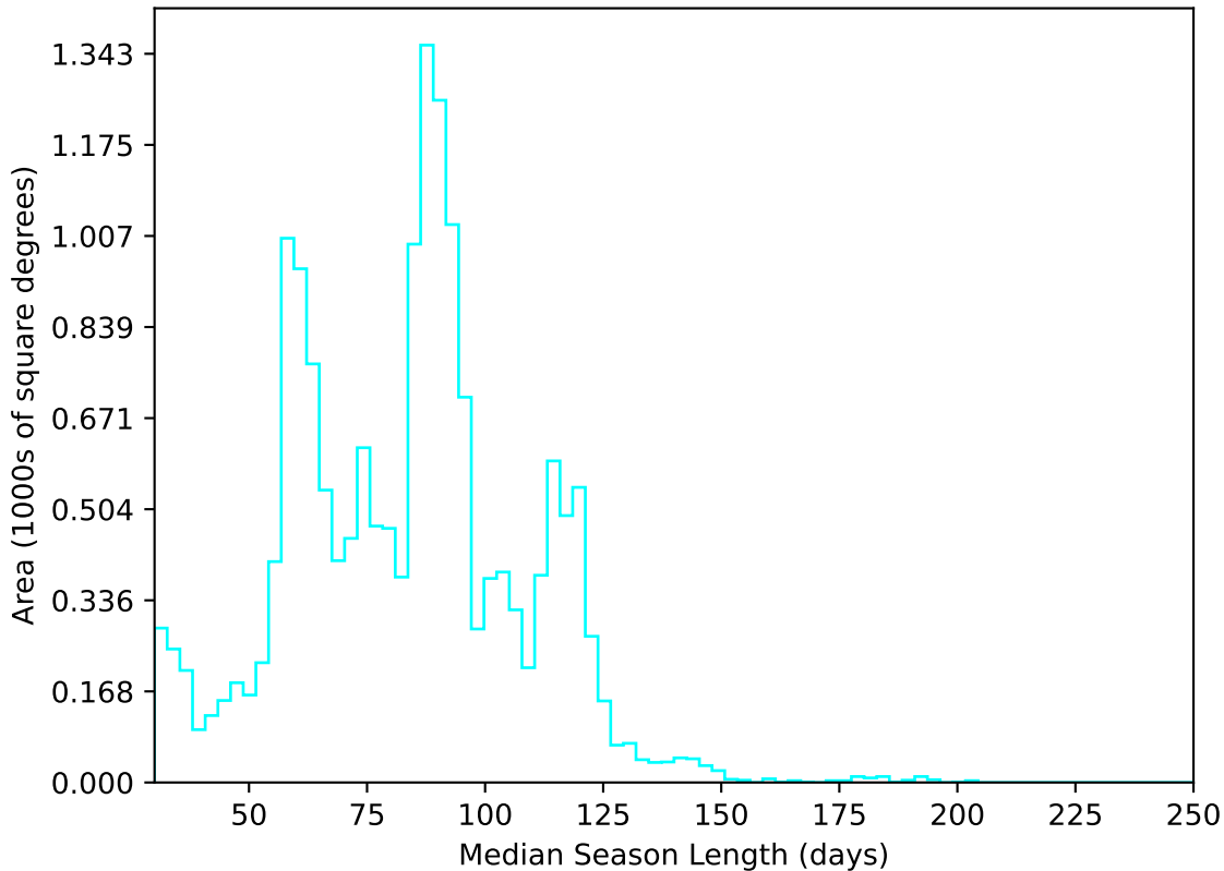
too_elab_r32_d3_griz_v3.4_10yrs WFD u band: Median Season Length
