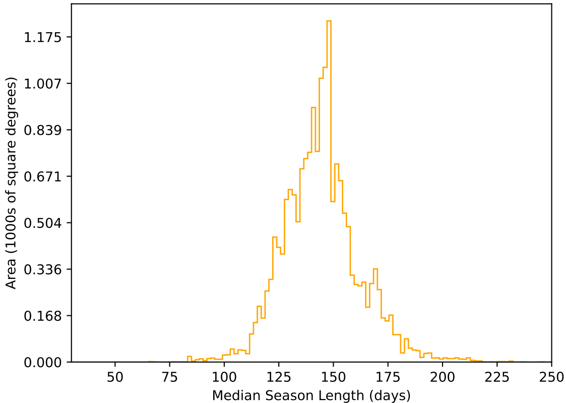
too_elab_r32_d3_griz_v3.4_10yrs WFD r band: Median Season Length
