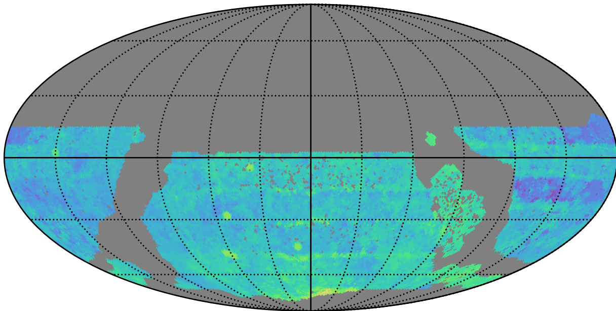
too_elab_r32_d3_griz_v3.4_10yrs WFD i band: Median Season Length
