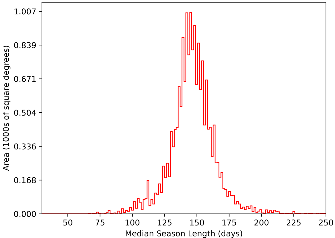
too_elab_r32_d3_griz_v3.4_10yrs WFD i band: Median Season Length
