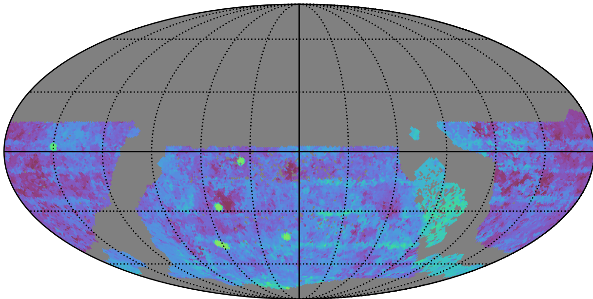
too_elab_r32_d3_griz_v3.4_10yrs WFD g band: Median Season Length
