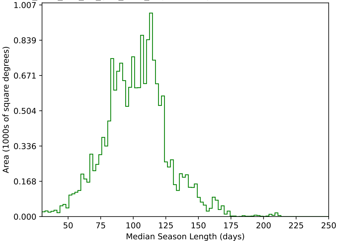
too_elab_r32_d3_griz_v3.4_10yrs WFD g band: Median Season Length
