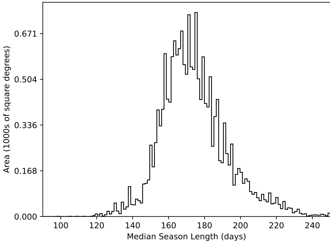
too_elab_r32_d3_griz_v3.4_10yrs WFD all bands: Median Season Length
