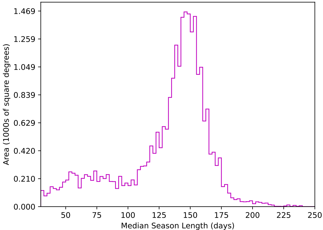
too_elab_r32_d3_griz_v3.4_10yrs All sky z band: Median Season Length
