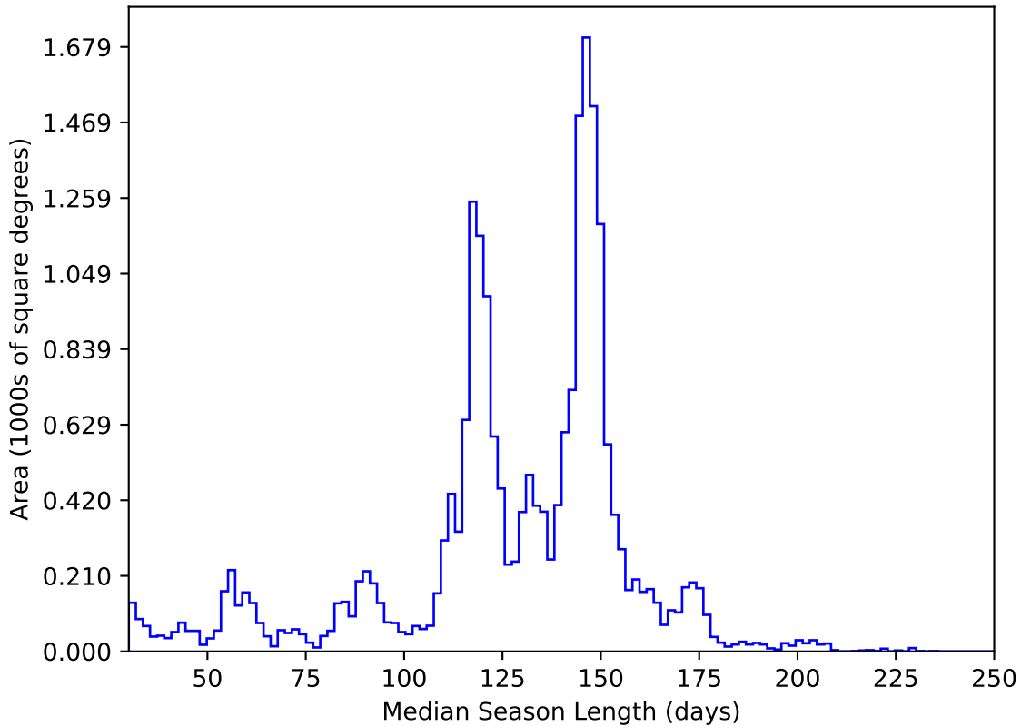
too_elab_r32_d3_griz_v3.4_10yrs All sky y band: Median Season Length
