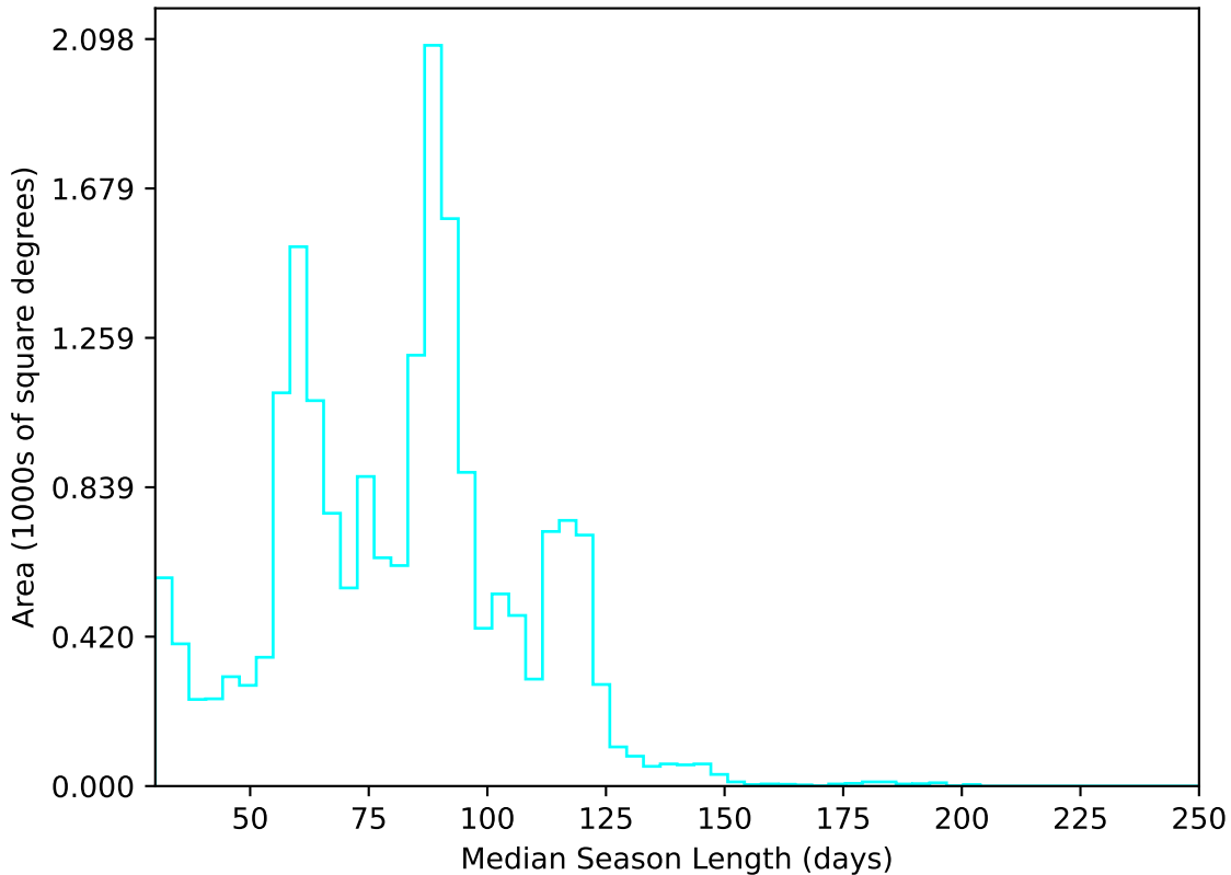
too_elab_r32_d3_griz_v3.4_10yrs All sky u band: Median Season Length
