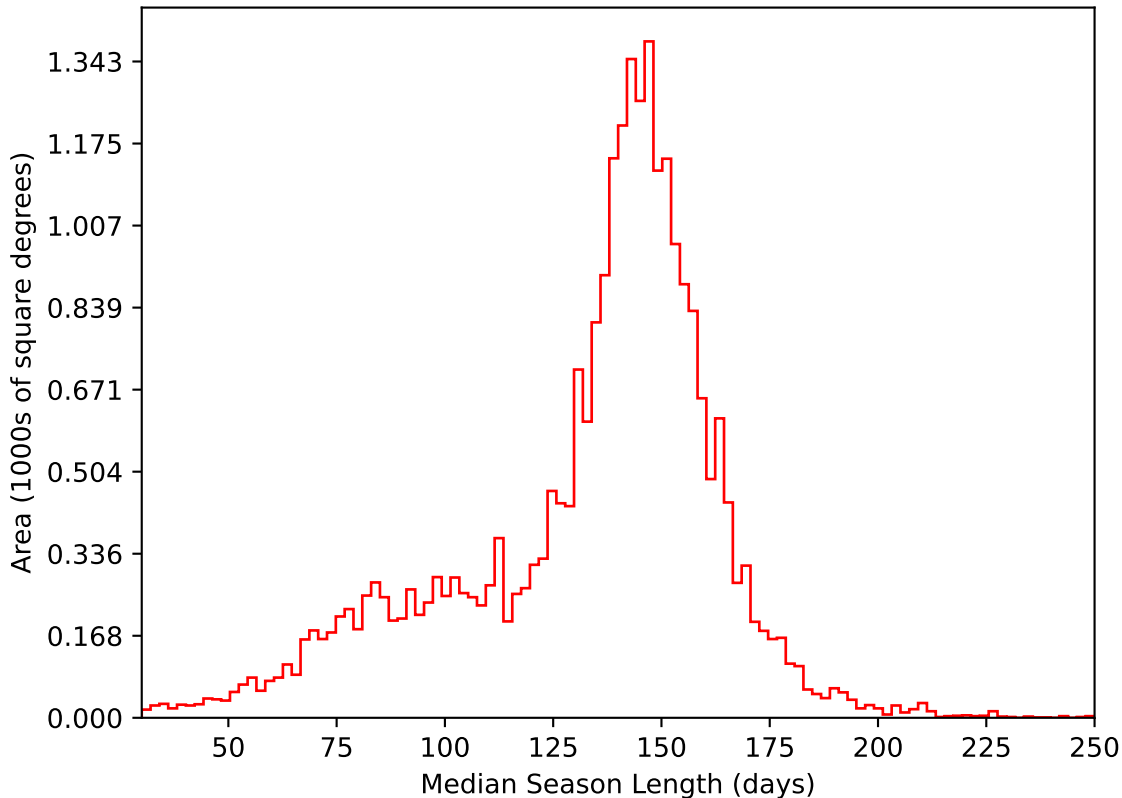
too_elab_r32_d3_griz_v3.4_10yrs All sky i band: Median Season Length
