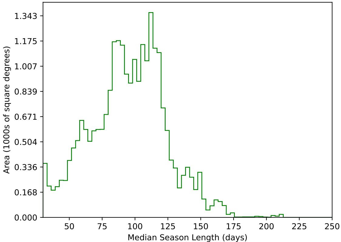
too_elab_r32_d3_griz_v3.4_10yrs All sky g band: Median Season Length
