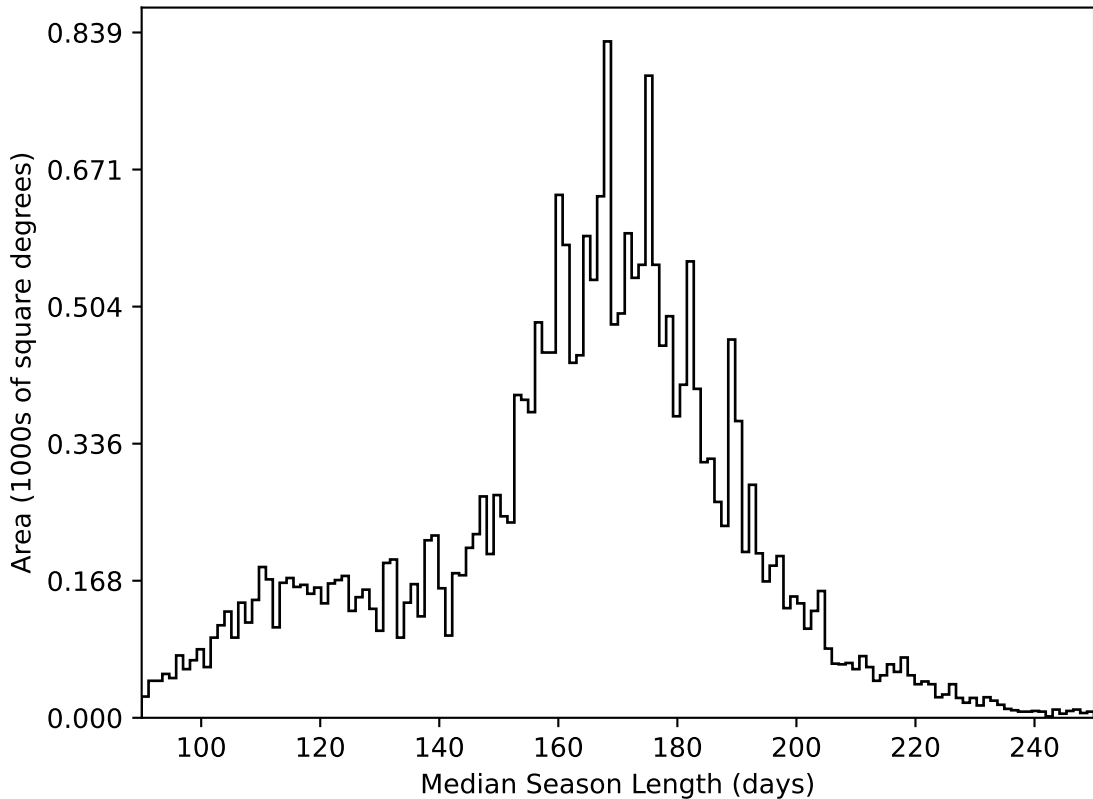
too_elab_r32_d3_griz_v3.4_10yrs All sky all bands: Median Season Length
