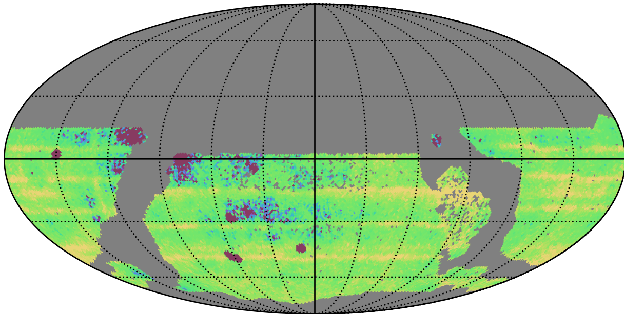
too_elab_r32_d3_griz_v3.4_10yrs WFD: Median Intra-Night Gap
