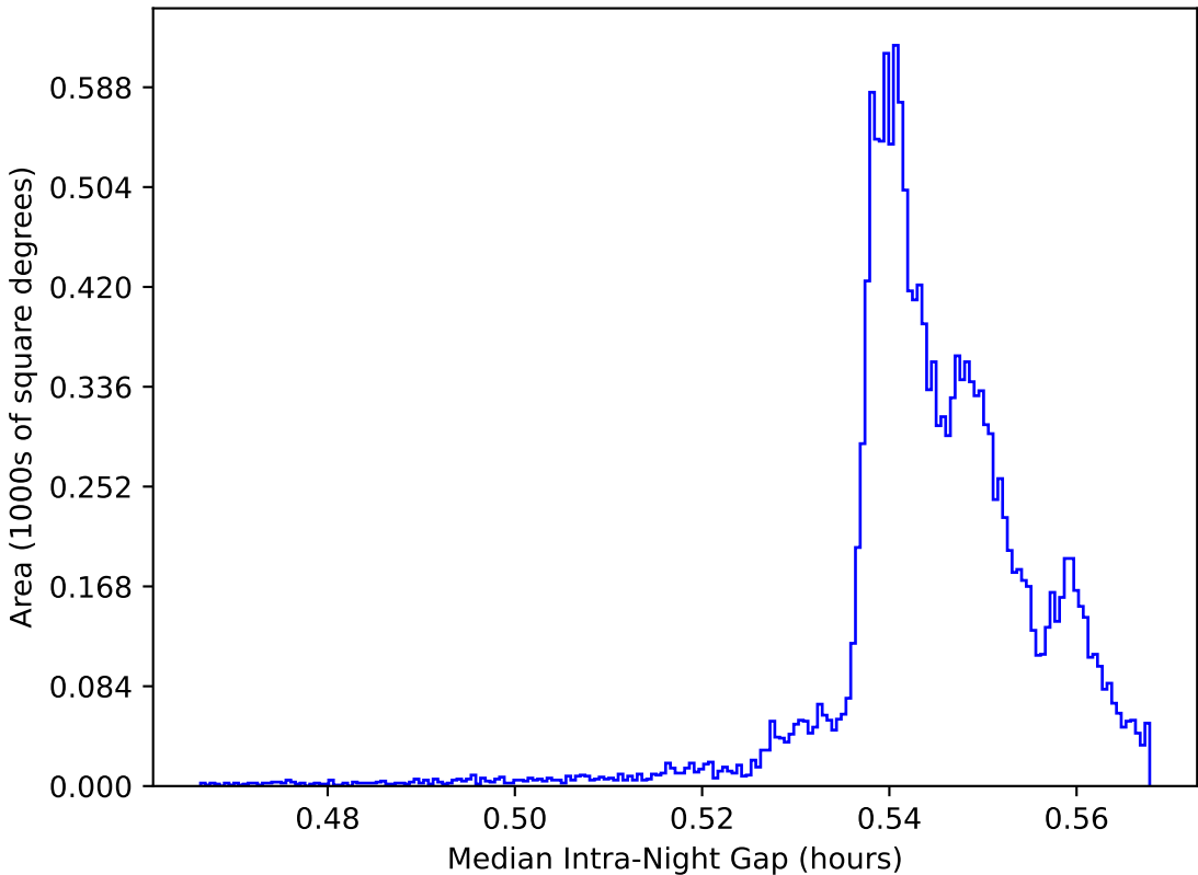
too_elab_r32_d3_griz_v3.4_10yrs WFD: Median Intra-Night Gap
