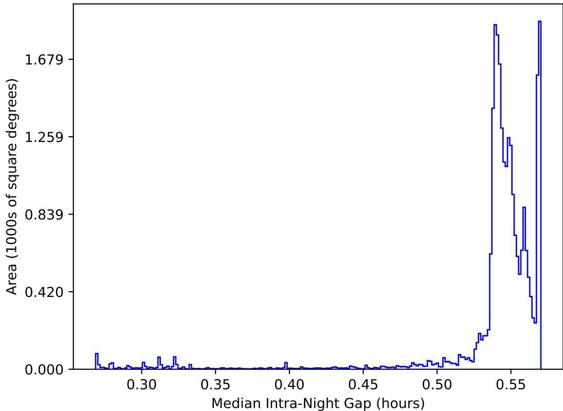
too_elab_r32_d3_griz_v3.4_10yrs All sky: Median Intra-Night Gap
