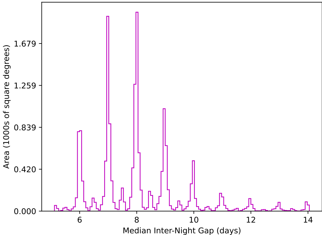
too_elab_r32_d3_griz_v3.4_10yrs WFD z band: Median Inter-Night Gap
