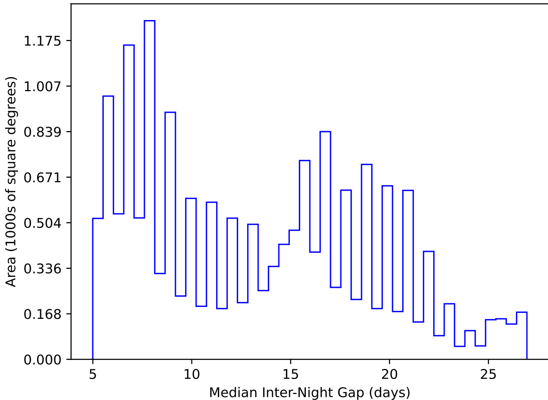
too_elab_r32_d3_griz_v3.4_10yrs WFD y band: Median Inter-Night Gap
