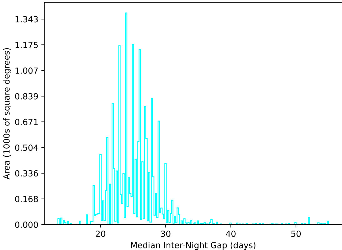
too_elab_r32_d3_griz_v3.4_10yrs WFD u band: Median Inter-Night Gap
