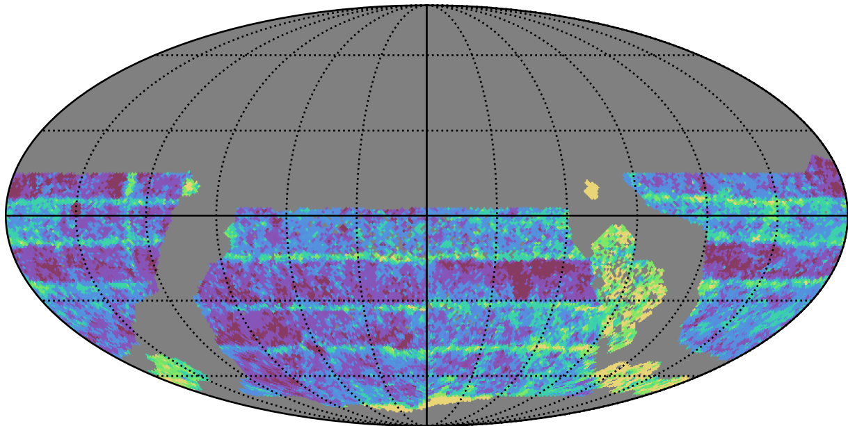
too_elab_r32_d3_griz_v3.4_10yrs WFD i band: Median Inter-Night Gap
