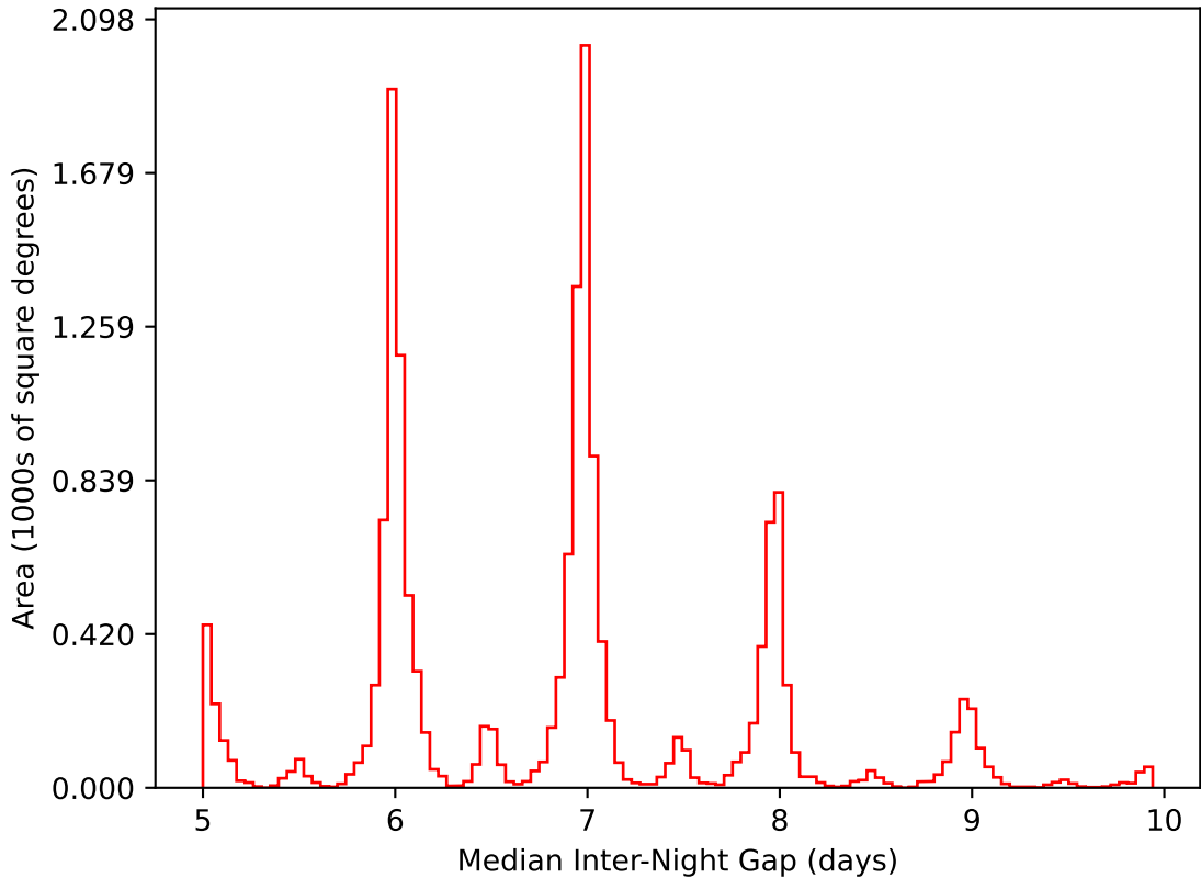
too_elab_r32_d3_griz_v3.4_10yrs WFD i band: Median Inter-Night Gap
