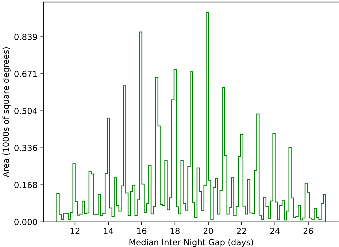
too_elab_r32_d3_griz_v3.4_10yrs WFD g band: Median Inter-Night Gap
