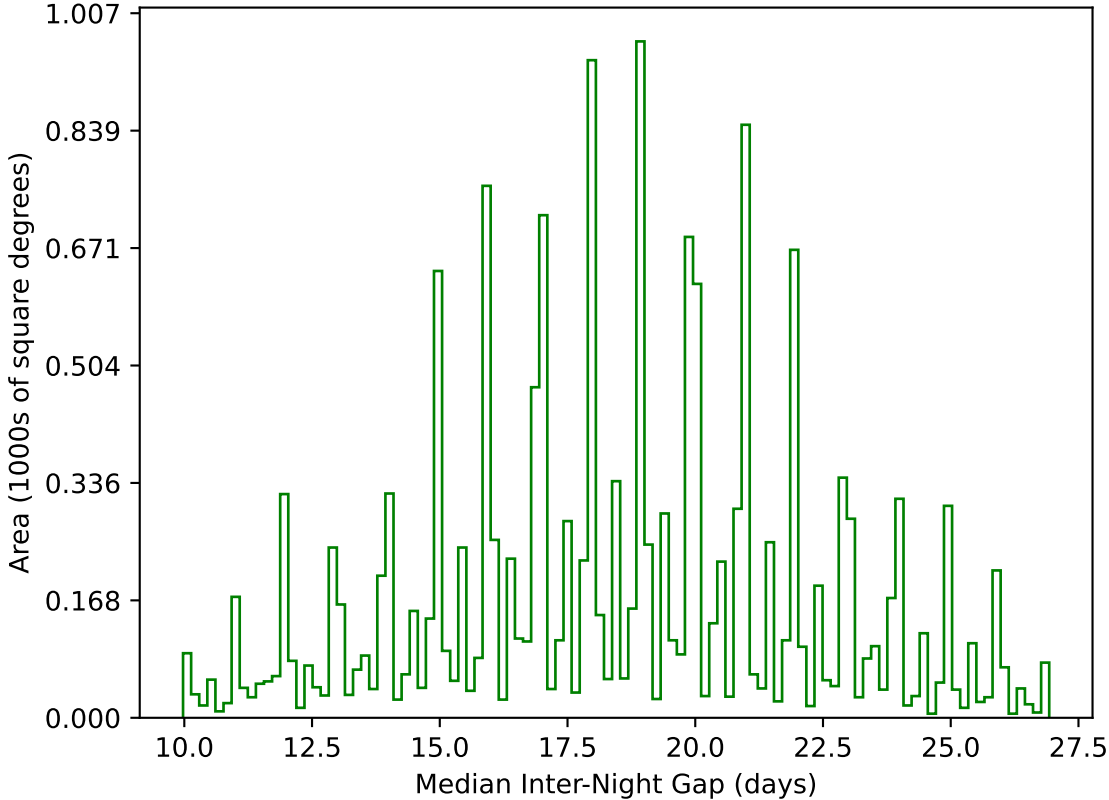
too_elab_r32_d3_griz_v3.4_10yrs WFD g band: Median Inter-Night Gap
