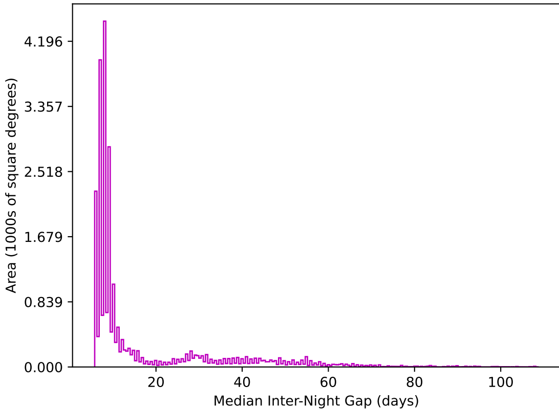
too_elab_r32_d3_griz_v3.4_10yrs All sky z band: Median Inter-Night Gap
