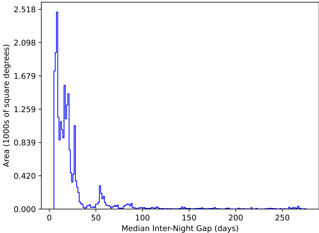
too_elab_r32_d3_griz_v3.4_10yrs All sky y band: Median Inter-Night Gap
