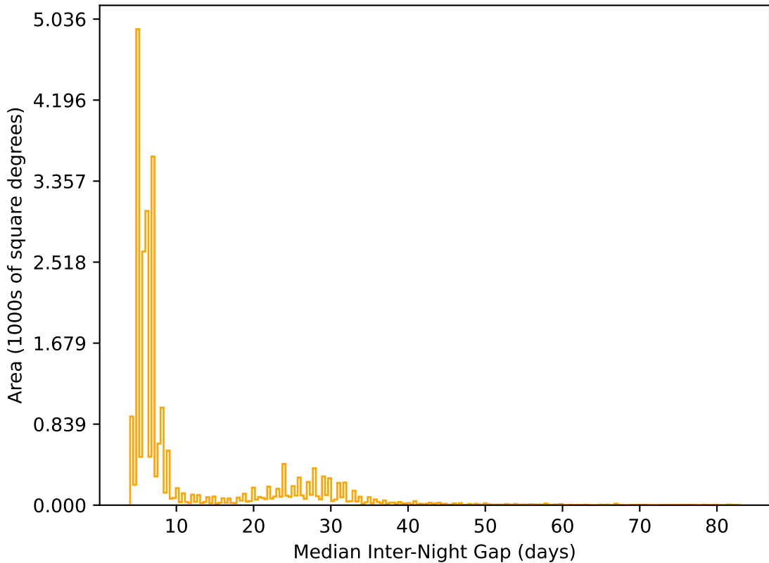
too_elab_r32_d3_griz_v3.4_10yrs All sky r band: Median Inter-Night Gap
