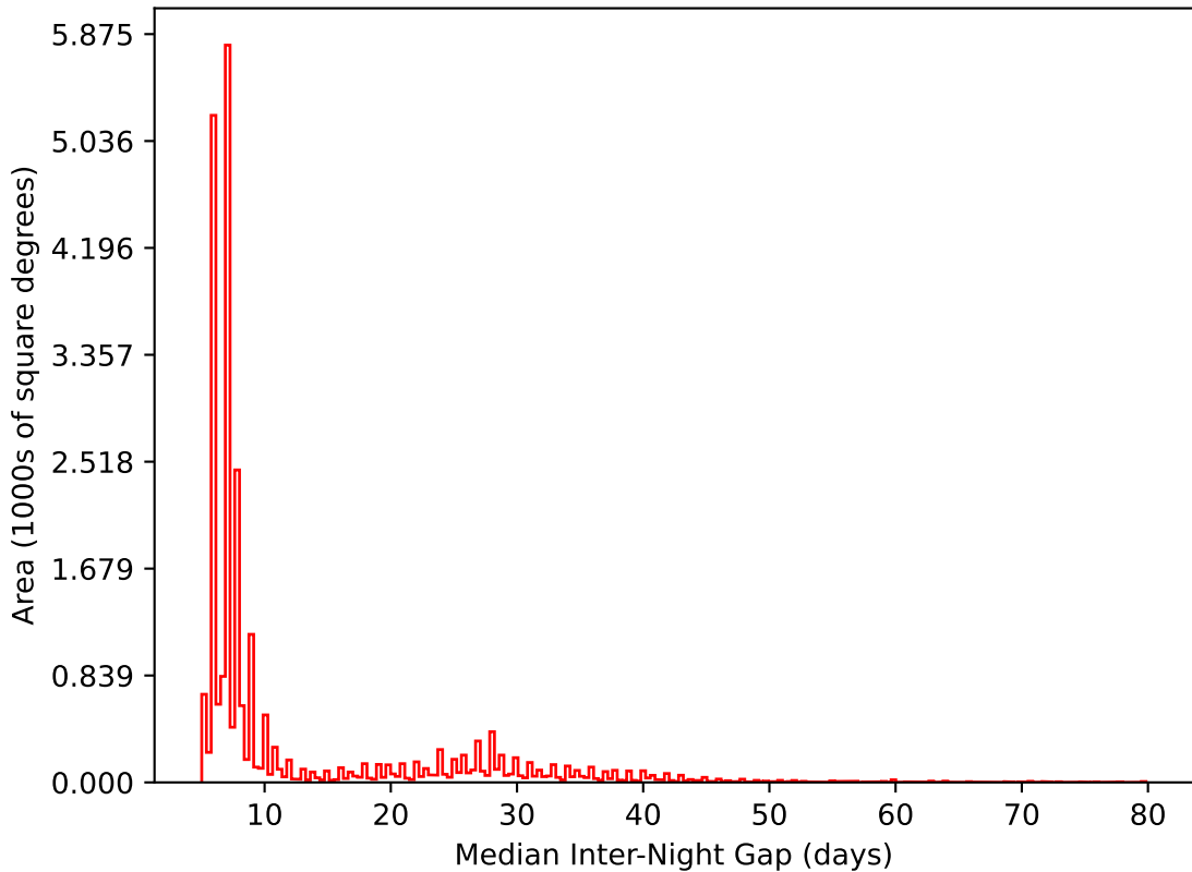
too_elab_r32_d3_griz_v3.4_10yrs All sky i band: Median Inter-Night Gap
