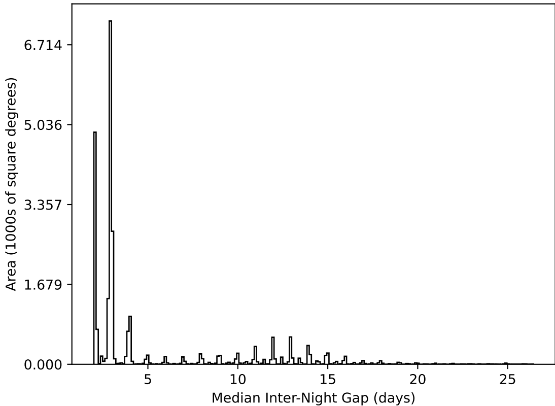
too_elab_r32_d3_griz_v3.4_10yrs All sky all bands: Median Inter-Night Gap
