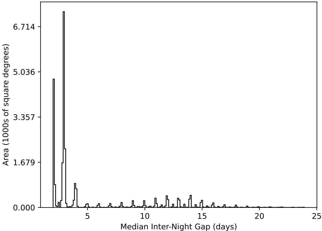
too_elab_r32_d3_griz_v3.4_10yrs All sky all bands: Median Inter-Night Gap
