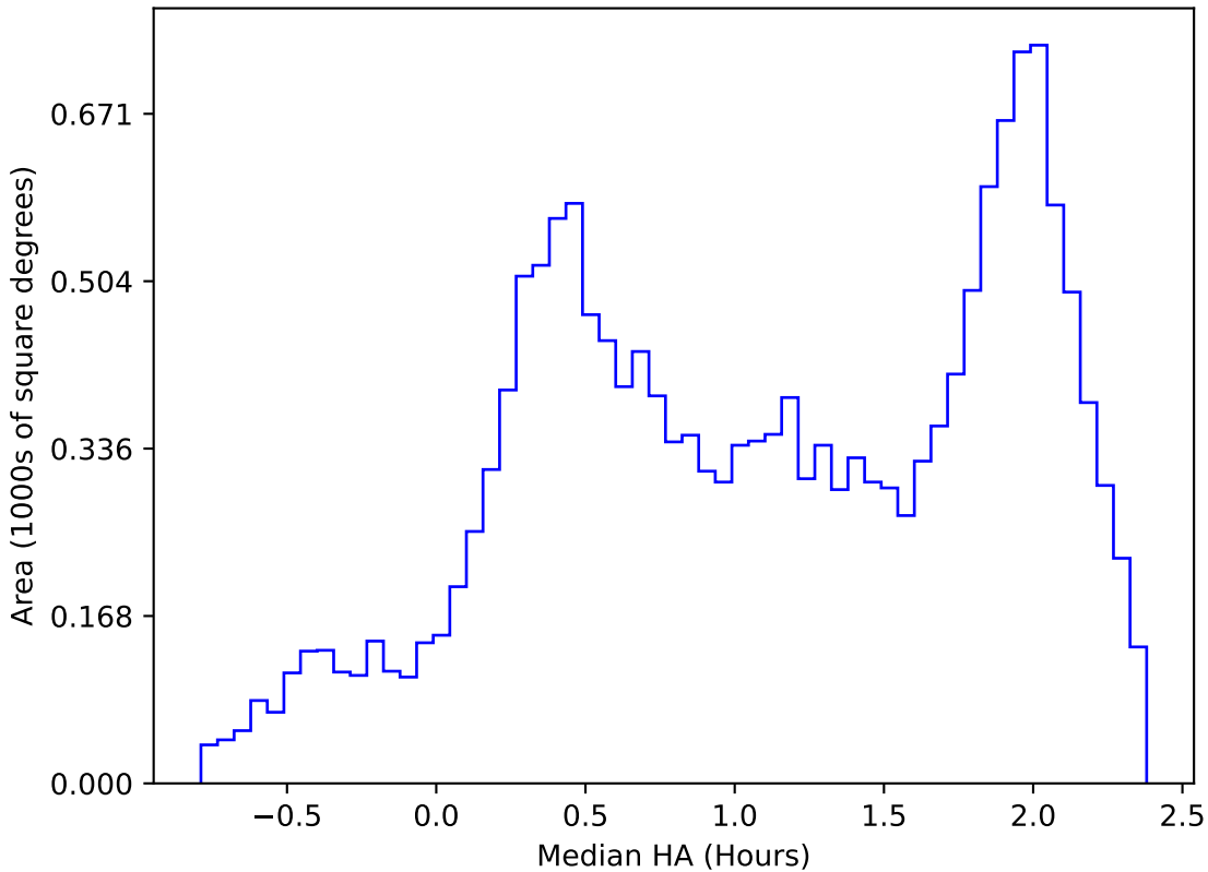
too_elab_r32_d3_griz_v3.4_10yrs WFD z band: Median HA
