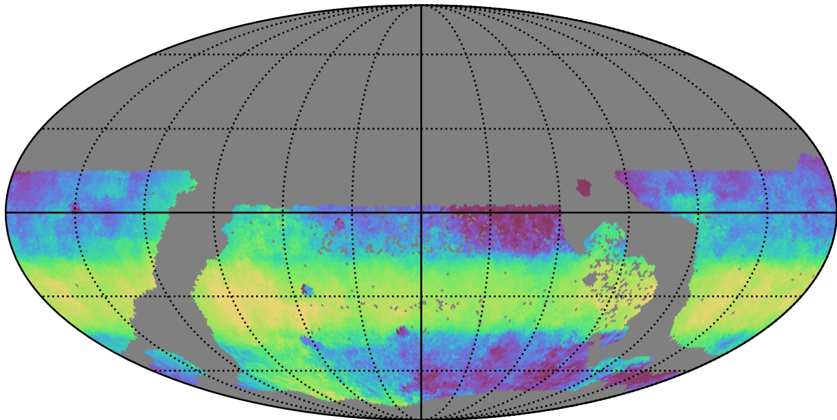
too_elab_r32_d3_griz_v3.4_10yrs WFD y band: Median HA
