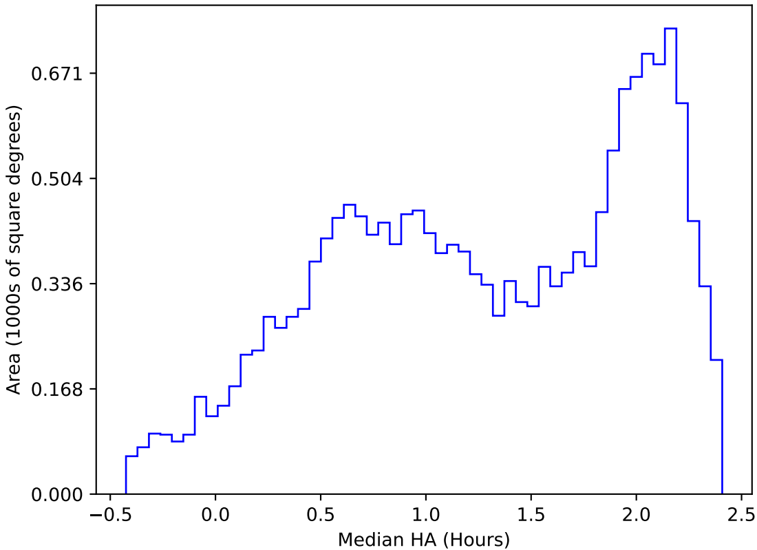
too_elab_r32_d3_griz_v3.4_10yrs WFD y band: Median HA
