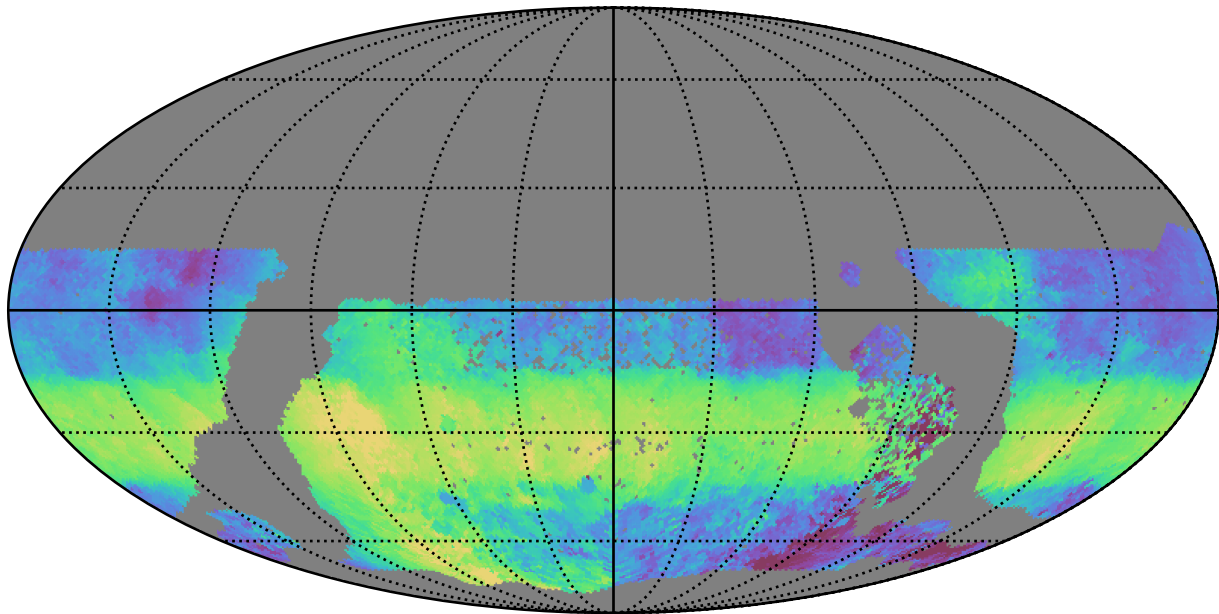
too_elab_r32_d3_griz_v3.4_10yrs WFD u band: Median HA
