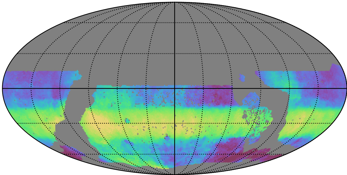
too_elab_r32_d3_griz_v3.4_10yrs WFD r band: Median HA
