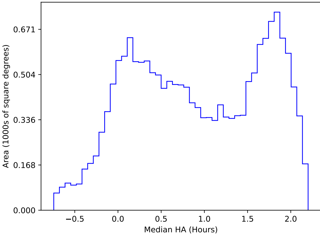
too_elab_r32_d3_griz_v3.4_10yrs WFD r band: Median HA
