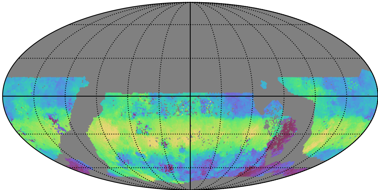
too_elab_r32_d3_griz_v3.4_10yrs WFD g band: Median HA
