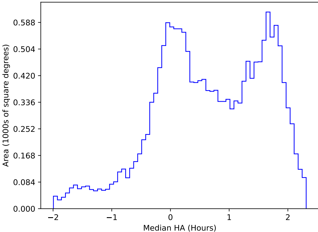
too_elab_r32_d3_griz_v3.4_10yrs WFD g band: Median HA
